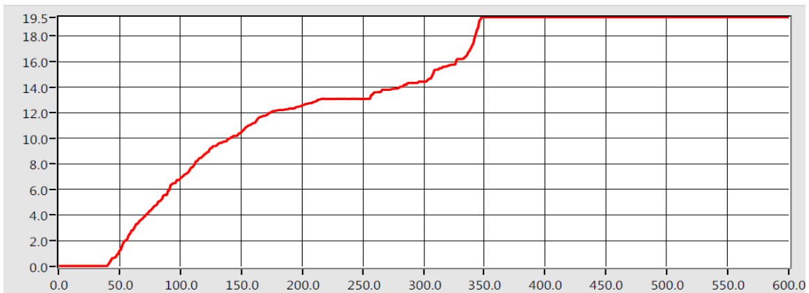
Graph No. 1 - Flame Spread Distance (ft) Versus Time (sec)
