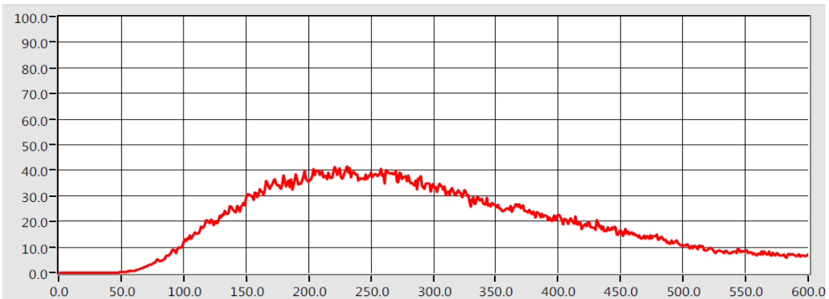
Graph No. 2 - Light Obscuration (%) Versus Time (sec)
